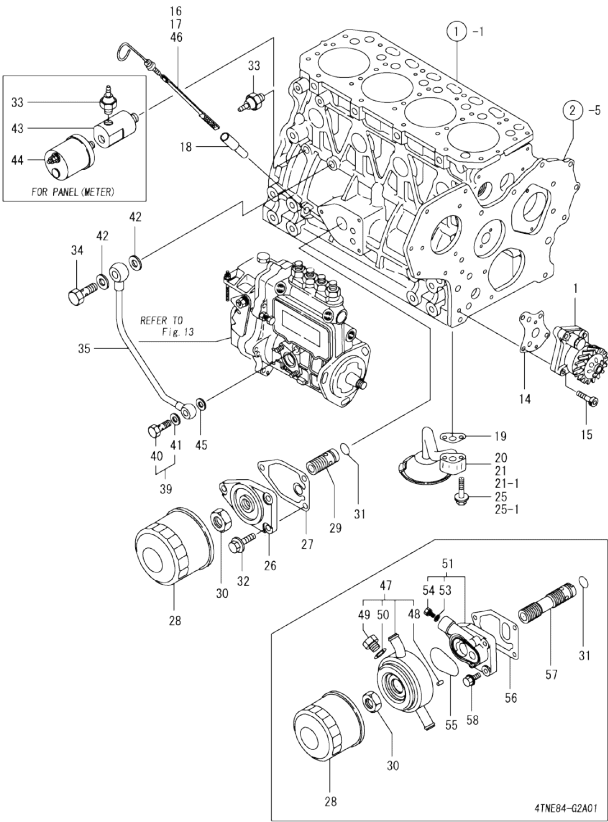
Fig.10. LUB.OIL SYSTEM
